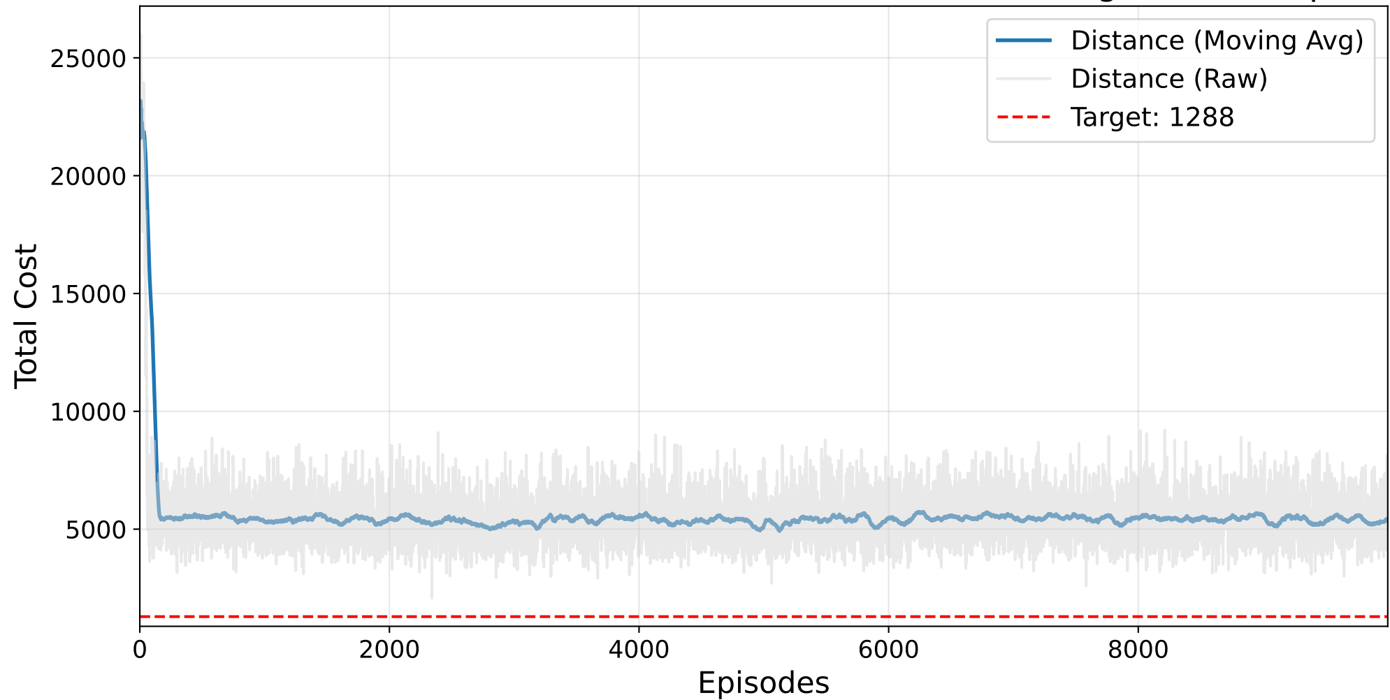
Final GAUSSIAN PROCESS Masked AutoRL-SOP Training - ESC47.sop
